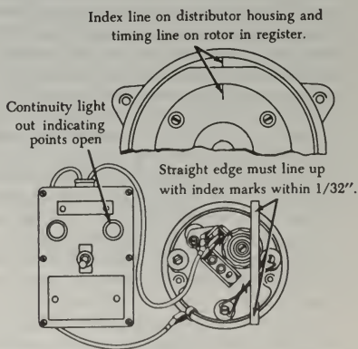
FIGURE 4-42. Scale in position for checking E-gap.
